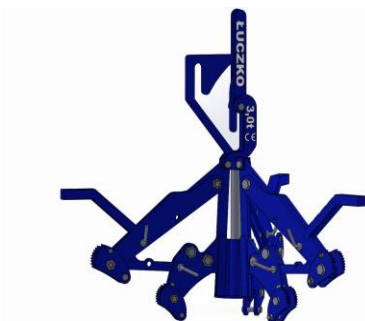
Gripping range 600-1500 mm Permissible work load 3000 kg weight 100kg
